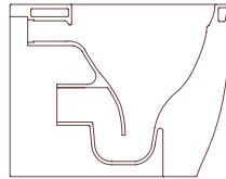
Art. 5205/TW GLAM TWIST WC - 55 x 36 Cm - 22 Kg
