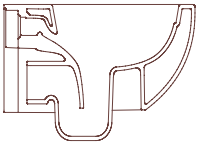
Art. 5203/TW GLAM TWIST HUNG WC - 55 x 36 Cm - 20 Kg
